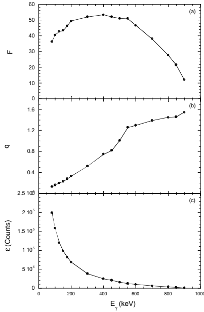
Figure 4.42: same as fig. 4.41 but for the 20.8 eV resonance
