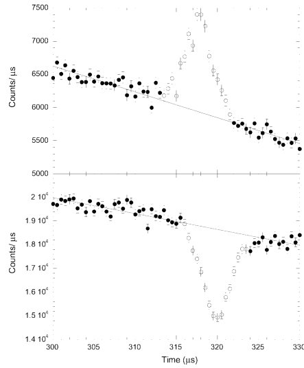
Figure 4.3: Neutron TOF spectra from a Pb sample recorded using a 30\ \mu\text{m} thick uranium foil in the experimental set-up of Figure 4.1. The NaI spectrum (top) has a peak corresponding to the Pb recoil peak at a final neutron energy of 6.67 eV. The same resonance gives rise to the absorption dip in the {}^6\text{Li} -glass spectrum (bottom).
