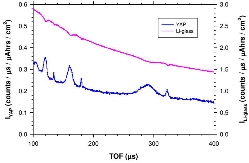
Figure 4.32: DINS spectra from a ZrH_2 sample acquired with a {}^6Li -glass detector (upper plot) and YAP scintillator (lower plot) placed at the sample scattering angle
