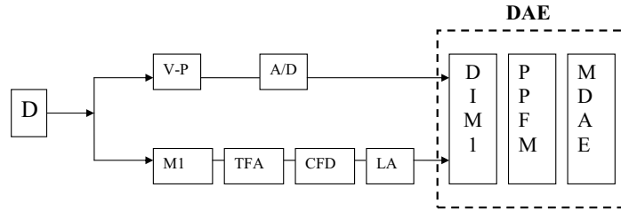
Figure 3.6: schematic of the RF (upper) and RD (lower) electronic chains
