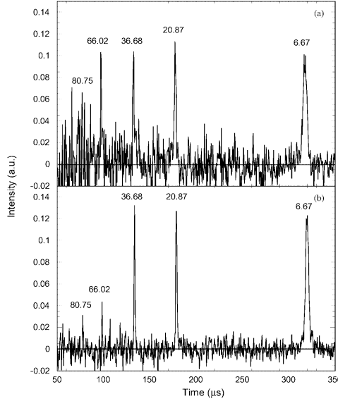
Figure 4.4: (a) Background corrected TOF spectrum from Pb recorded by the NaI with a 30\ \mu\text{m} ^{238}\text{U} foil. The spectrum is normalised so that the area under the 6.67 eV peak amounts to one count; (b) Same as (a) but recorded by the ^6\text{Li} glass scintillator. Normalisation is the same as for case (a).
