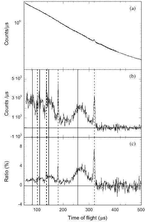
Figure 4.11: (a) Neutron TOF spectra from a 50% {}^4\text{He} - \text{H}_2 mixture measured with 120 \mu\text{m} thick {}^{238}\text{U} foil; (b) difference spectrum; (c) ratio of the difference spectrum (b) to the spectrum in (a).
