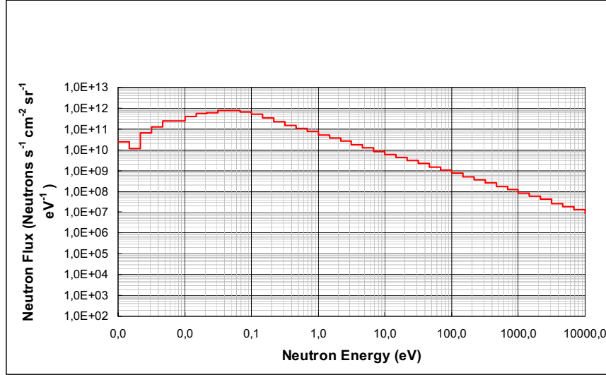
Figure 2.5: Incident neutron energy spectrum of the VESUVIO spectrometer.
