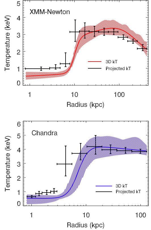
Fig. 8: Projected radial ICM temperature values plotted over the deprojected temperature profiles corresponding to r = 12.5' for XMM-Newton (top) and r = 4' for Chandra (bottom) as described in Sect. 3.2. Confidence envelopes for XMM-Newton (red) and Chandra (blue) were propagated from Monte Carlo realizations of the fit analytical functions.
