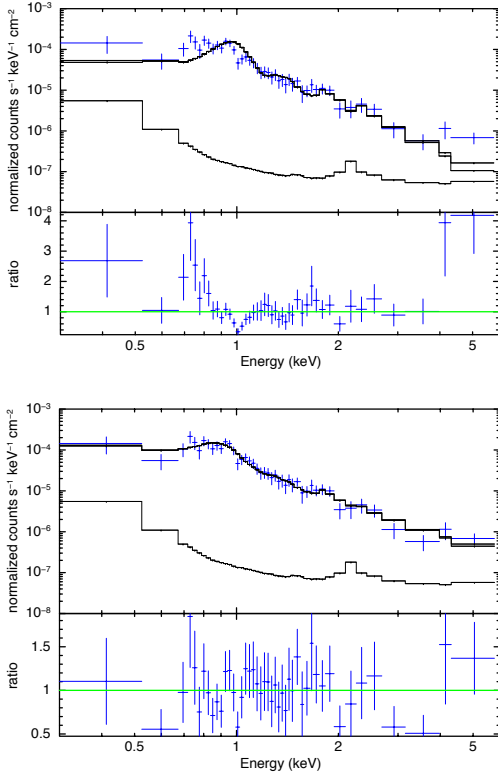
Fig. 11: Chandra spectral fitting of r = 3 kpc circular region centered at NGC 5718 with Model 1 (upper) and Model 2 (lower). For plotting purposes only, adjacent bins are combined until they have a significant detection at least as large as 2\sigma , with maximum 5 bins. Upper curve corresponds to the simultaneous fit of the Chandra ACIS-I source and background counts, where the lower curve presents the background model.
