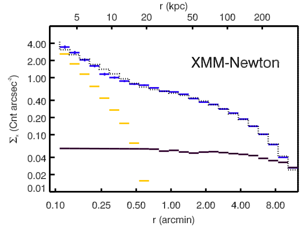
Fig. 6: XMM-Newton surface brightness fitting with double \beta -model in 0.5 - 2.5 keV energy band in circular region with r = 12.5' . Background (black); XMM-Newton point spread function model (yellow); surface brightness of the cluster (blue); the double \beta -model fit of the projected surface brightness (dotted black curve).
