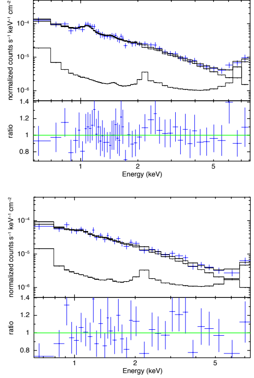
Fig. C.1: Chandra spectral fitting of Sector 1 (upper) and Sector 2 (lower) with phabs \times apec models. For plotting purposes only, adjacent bins are combined until they have a significant detection at least as large as 5\sigma , with maximum 10 bins. Upper curve corresponds to the simultaneous fit of the Chandra ACIS-I source and background counts, where the lower curve presents the background model in each panel.
