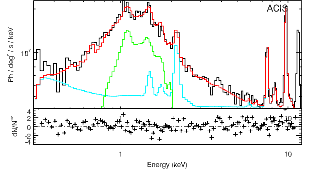
Fig. 3: Chandra ACIS-I background fitting of three combined observations. Total number of counts (black); quiescent particle background emission (cyan); cluster emission (green); total background emission (red). Residuals correspond to the total photon count with respect to the ICM and total background emission.
