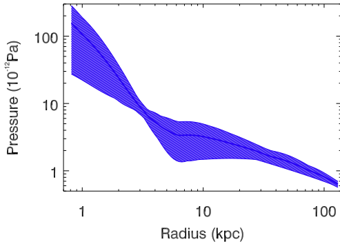
Fig. 9: Hot gas pressure profile centered at BCG.
