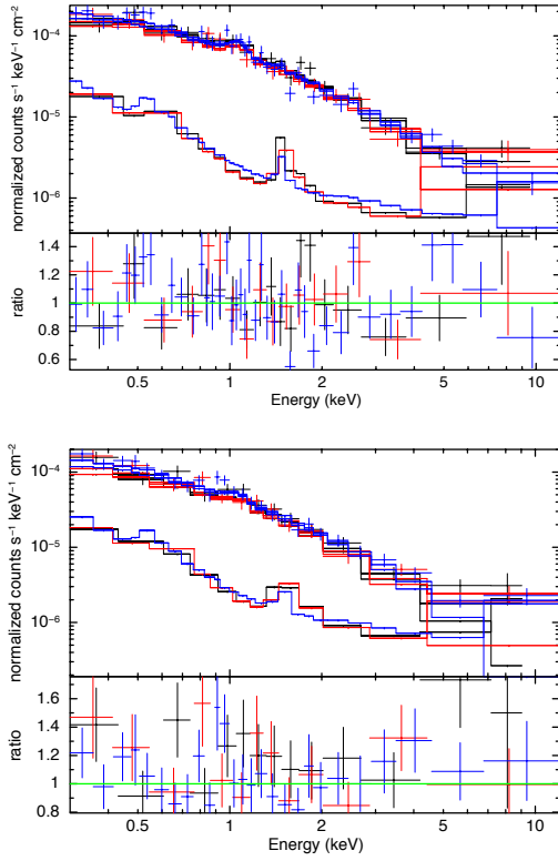
Fig. C.2: Same as Fig. C.1, but for XMM-Newton EPIC spectra.
