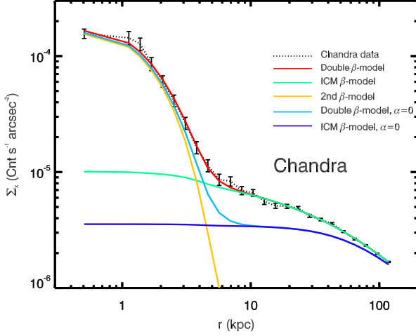
Fig. 7: Chandra surface brightness fit of double \beta -model in 0.5 - 2.5 keV energy band in circular region with r = 4' . Projected surface brightness (dotted black curve); the double \beta -model (red); the \beta -model corresponding to the ICM (green); the second \beta -model corresponding to the corona (yellow); the double \beta -model with \alpha parameter is set to zero (light blue); the \beta -model of the ICM with \alpha parameter is set to zero (dark blue).
