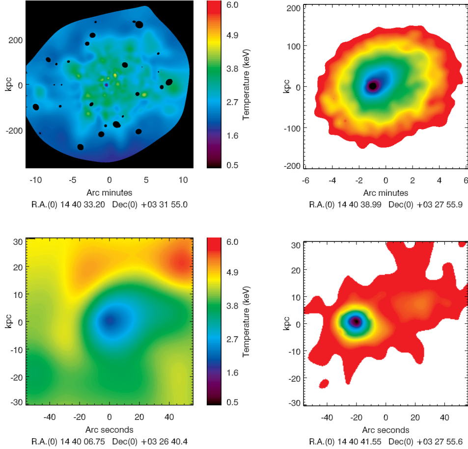
Fig. 4: Upper panel : XMM-Newton temperature map ( left ) and surface brightness map ( right ). Lower panel : For the highest angular resolution, Chandra temperature map ( left ) and surface brightness map ( right ). Temperature maps are presented within 3\sigma errors. Surface brightness maps are obtained in soft energy band 0.3-2.5 keV within 4\sigma errors. Chandra maps are enlarged to emphasize the central region of the cluster.
