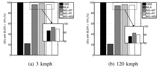
Fig. 9. # UEs with BLER < 10% for the Heavy Tree Shadowed environment.
