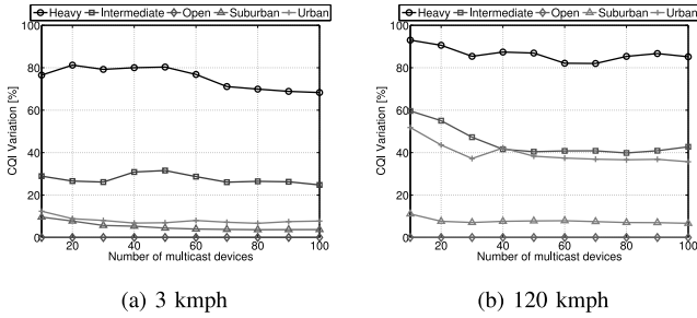
Fig. 8. Variation of user’ CQI for 3 kmph and 120 kmph.
