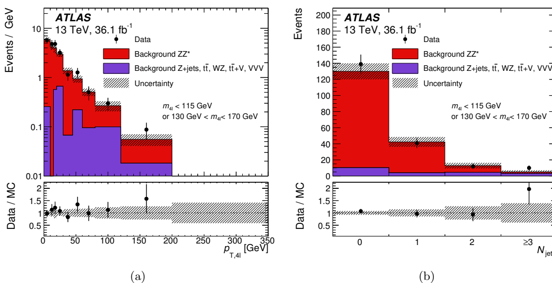
Figure 2. Reconstructed event yields in bins of (a) the transverse momentum of the four leptons p_{T,4\ell} and (b) the number of jets N_{\text{jets}} , in a non-resonant ZZ^* -enriched control region, obtained by applying the full event selection except for the m_{4\ell} window, i.e. m_{4\ell} < 115 \text{ GeV} or 130 \text{ GeV} < m_{4\ell} < 170 \text{ GeV} . The error bars on the data points indicate the statistical uncertainty. The uncertainty in the prediction is shown by the dashed band. The bottom part of the figures shows the ratio of data to the MC expectation.
