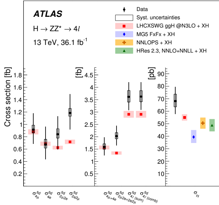
Figure 7. The fiducial cross sections (left two panels) and total cross section (right panel) of Higgs boson production measured in the 4\ell final state. The fiducial cross sections are shown separately for each decay channel, and for same- and opposite-flavour decays. The inclusive fiducial cross section is measured as the sum of all channels, as well as by combining the per-channel measurements assuming SM ZZ^* \rightarrow 4\ell branching ratios. The LHCXSWG prediction is accurate to N3LO in QCD for the ggF process. For the fiducial cross-section predictions, the LHCXSWG cross sections are multiplied by the acceptances determined using the NNLOPS sample for ggF and the samples discussed in section 3 for the other production modes. For the total cross section, the cross-section predictions by the generators NNLOPS, HRES, and MG5_AMC@NLO_FxFx are also shown. The cross sections for all other Higgs boson production modes XH are added. The error bars on the data points show the total uncertainties, while the systematic uncertainties are indicated by the boxes. The shaded bands around the theoretical predictions indicate the PDF and scale uncertainties.
