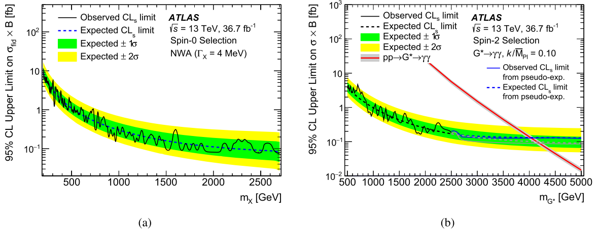
Fig. 4. (a) Upper limits on the fiducial cross section times branching ratio to two photons at \sqrt{s} = 13 TeV of a narrow-width ( \Gamma_X = 4 MeV) spin-0 resonance as a function of its mass m_X . (b) Upper limits on the production cross section times branching ratio to two photons at \sqrt{s} = 13 TeV of the lightest KK graviton as a function of its mass m_{G^*} for k/\overline{M}_{Pl} = 0.1 . For m_{G^*} > 2500 GeV, the observed and expected limits are determined with pseudo-experiments shown by the blue solid and dashed lines, respectively. Predictions are shown for the RS1 model, where the grey shaded band represents the PDF uncertainty. (For interpretation of the references to colour in this figure legend, the reader is referred to the web version of this article.)
