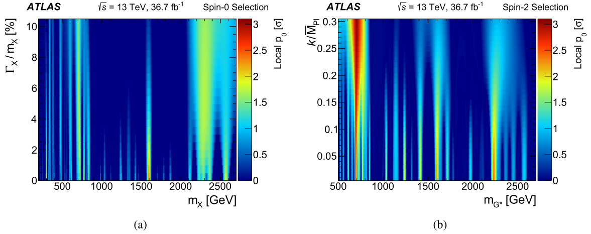
Fig. 3. Compatibility, in terms of local p_0 quantified in standard deviations \sigma , with the background-only hypothesis (a) as a function of the assumed signal mass m_X and relative width \Gamma_X/m_X for the spin-0 resonance search and (b) as a function of the assumed signal mass m_{G^*} and k/\overline{M}_{Pl} for the spin-2 resonance search. Only positive excesses are considered.
