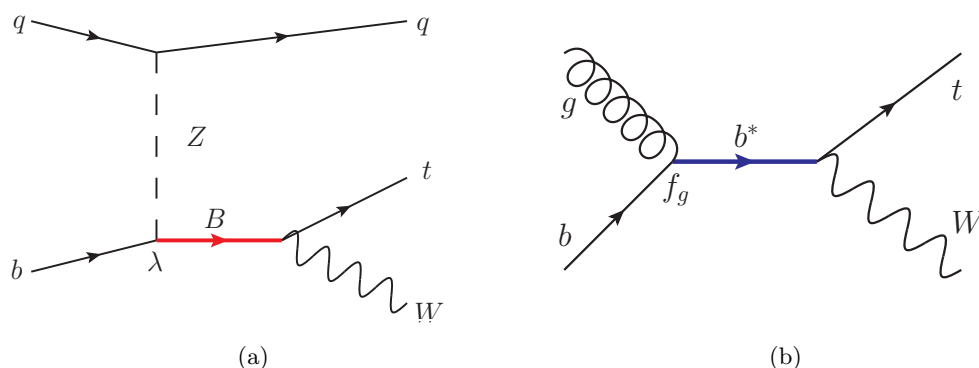
Figure 1. Leading-order Feynman diagrams for the production and decay of (a) a single B together with a light quark and (b) a single b^* .
