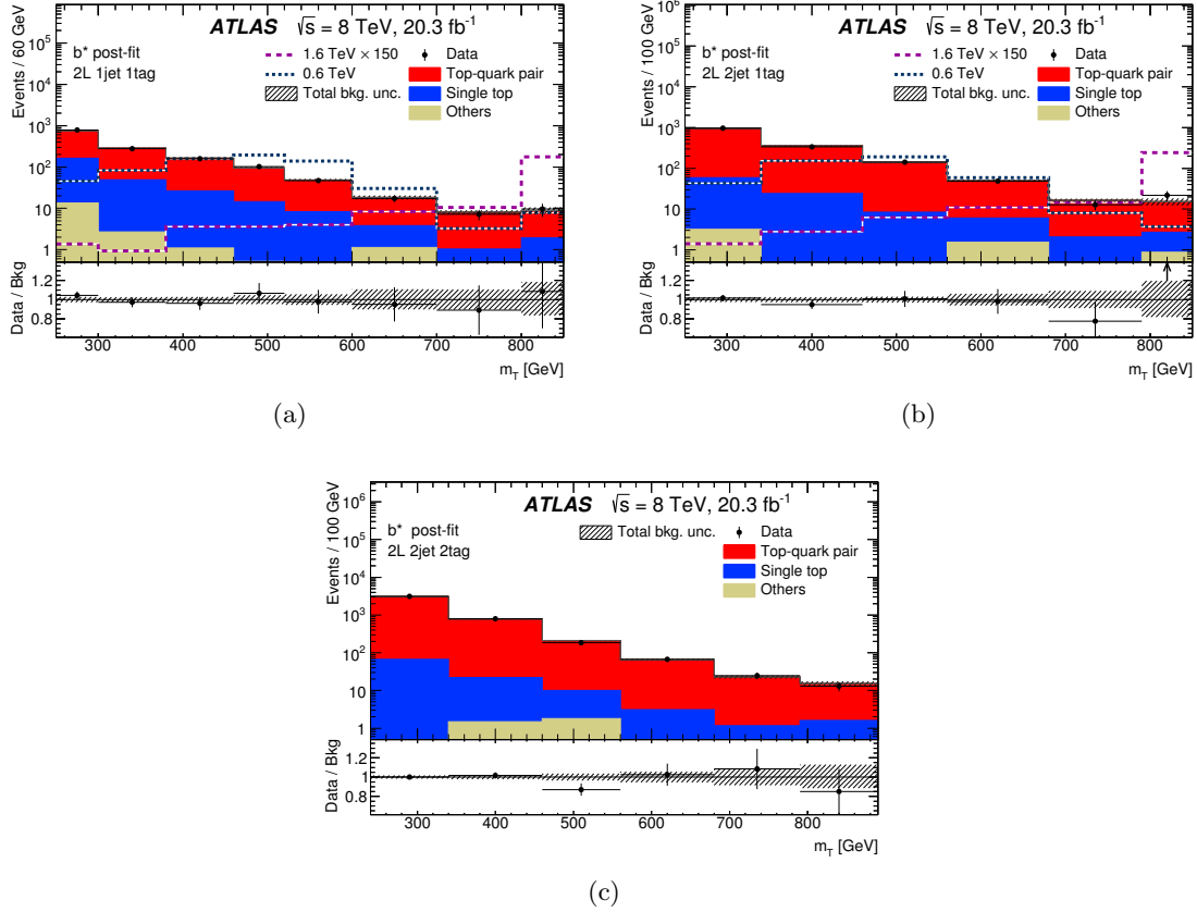
Figure 11. Distributions of the discriminant variable, transverse mass, m_T , in the dilepton channel for data and SM background processes in the (a) 2L\ 1jet\ 1tag signal region, (b) 2L\ 2jet\ 1tag signal region and (c) 2L\ 2jet\ 2tag control region using the b^* selection. For the signal region distributions, the two included b^* signal distributions are scaled to the theory cross-sections multiplied by the indicated factor for better visibility. The background processes are normalised to their post-fit normalisation. The uncertainty band includes statistical and all systematic uncertainties. The first and the last bin contain the underflow and overflow, respectively. The binning of the figures is the same as used in the binned likelihood fit function.
