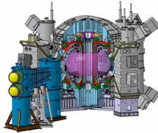
Image: JT-60SA
