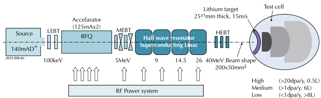
Image: IFMIF/EVEDA
