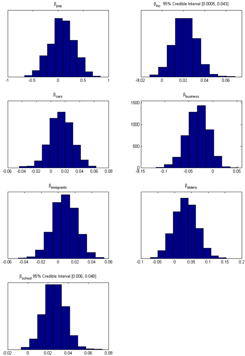
Figure 13: House price data: posterior estimation of \beta .
