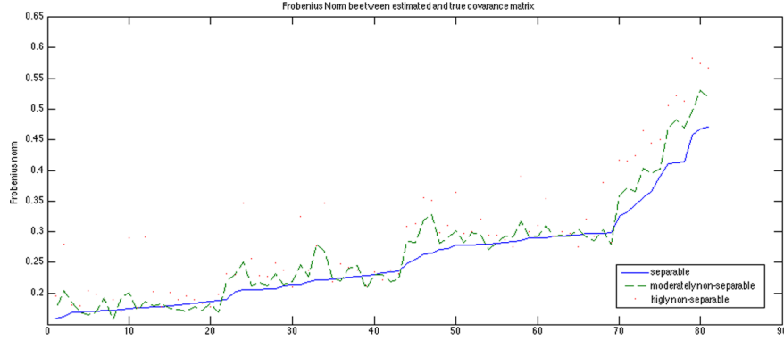
Figure 14: Frobenius norm of the distance between the true non separable matrix \Sigma and the matrix \hat{\Psi} \otimes \hat{\Phi} estimated assuming the unstructured conditionally separable model and for different choices of the parameters defining \Sigma .
