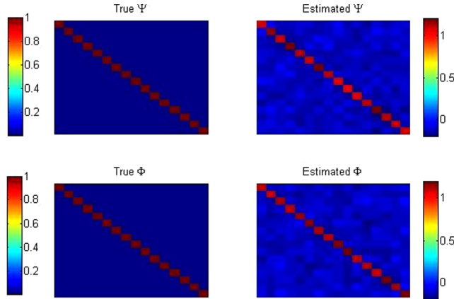
Figure 4: Posterior estimation of \Phi and \Psi : unstructured model, T = 16 , N = 16 . The true \Psi matrix is I_T , the true \Phi is I_N .
