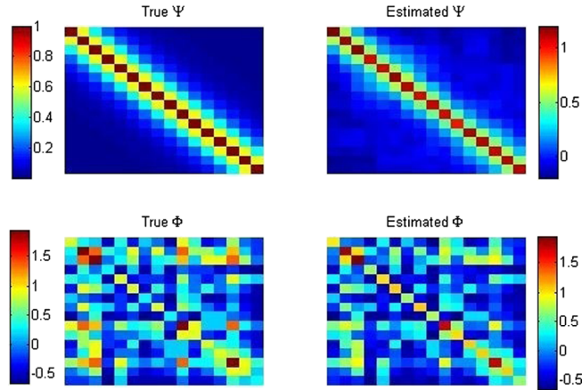
Figure 1: Posterior estimation of \Phi and \Psi : unstructured model. T = 16 , N = 16 . The true \Psi matrix is AR(1) with parameter \rho = 0.6 , the true \Phi is Expn(\lambda \mathbf{W}) , with \lambda = 0.6 .
