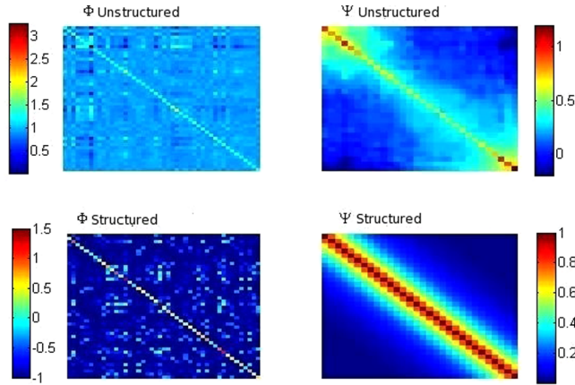
Figure 6: Cigarette Example: posterior estimation of temporal and spatial covariance matrices under structured and unstructured models, space and time fixed effects included.
