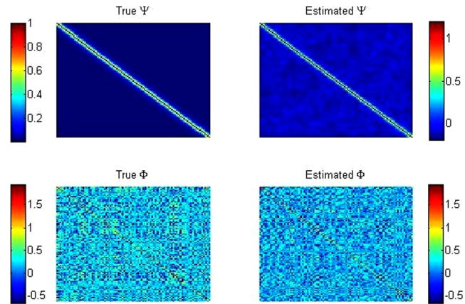
Figure 2: Posterior estimation of \Phi and \Psi : unstructured model. T = 100 , N = 100 . The true \Psi matrix is AR(1) with parameter \rho = 0.6 , the true \Phi is Expn(\lambda \mathbf{W}) , with \lambda = -0.6 .
