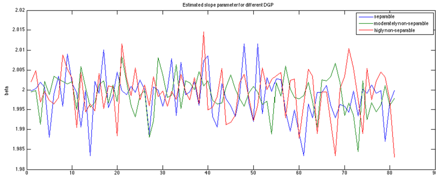
Figure 15: Posterior mean of \hat{\beta} from the estimation of all 243 different spatial error models following (20) estimated assuming the unstructured conditionally separable model ( \beta = 2 ).
