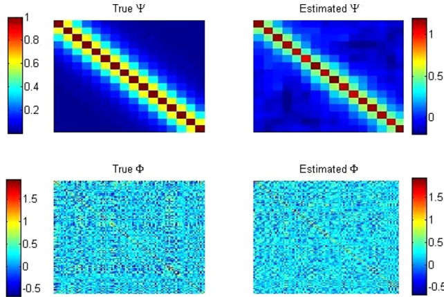
Figure 3: Posterior estimation of \Phi and \Psi : unstructured model. T = 16 , N = 100 . The true \Psi matrix is AR(1) with parameter \rho = 0.6 , the true \Phi is Exp_m(\lambda \mathbf{W}) , with \lambda = -0.6 .
