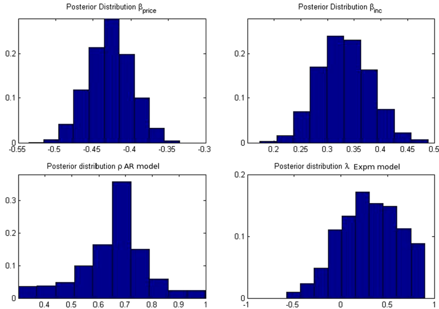
Figure 5: Cigarette Example: posterior distribution of \beta under unstructured separable model (with spatial and temporal effects) and posterior distribution of \rho and \lambda under AR and Expm models (with spatial and temporal effects), respectively.
