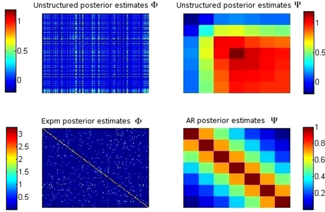
Figure 12: House price data: posterior estimation of matrices \Psi and \Phi under unstructured and structured models, without fixed effects.
