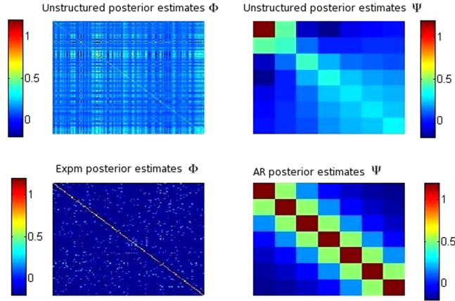
Figure 11: House price data: posterior estimation of matrices \Psi and \Phi under unstructured and structured models, space fixed effects included.
